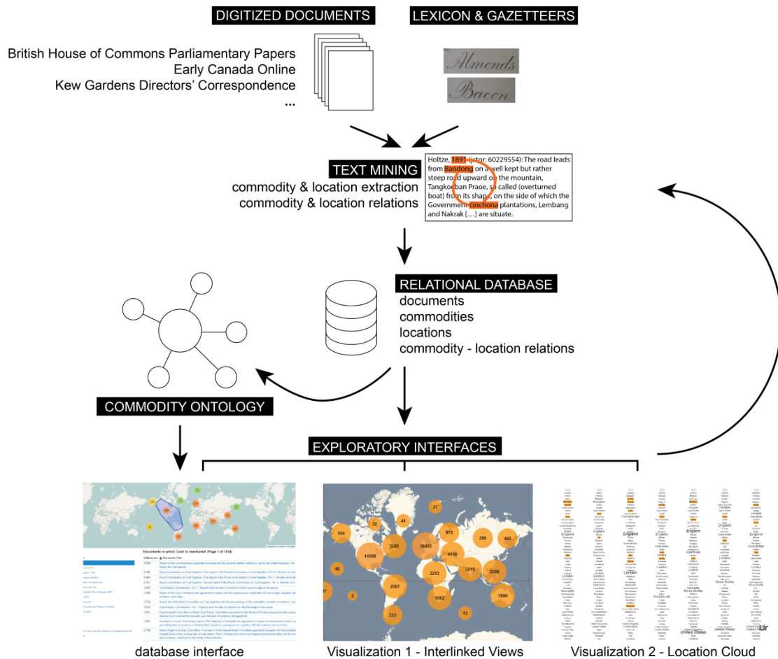
Figure 1: Technical Approach of Trading Consequences.
